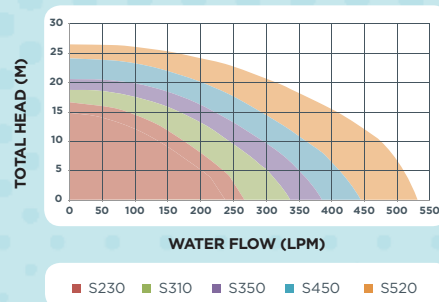
SUMMIT SERIES PERFORMANCE CURVES
